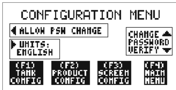
FIGURE 5-1 Configuration Menu
